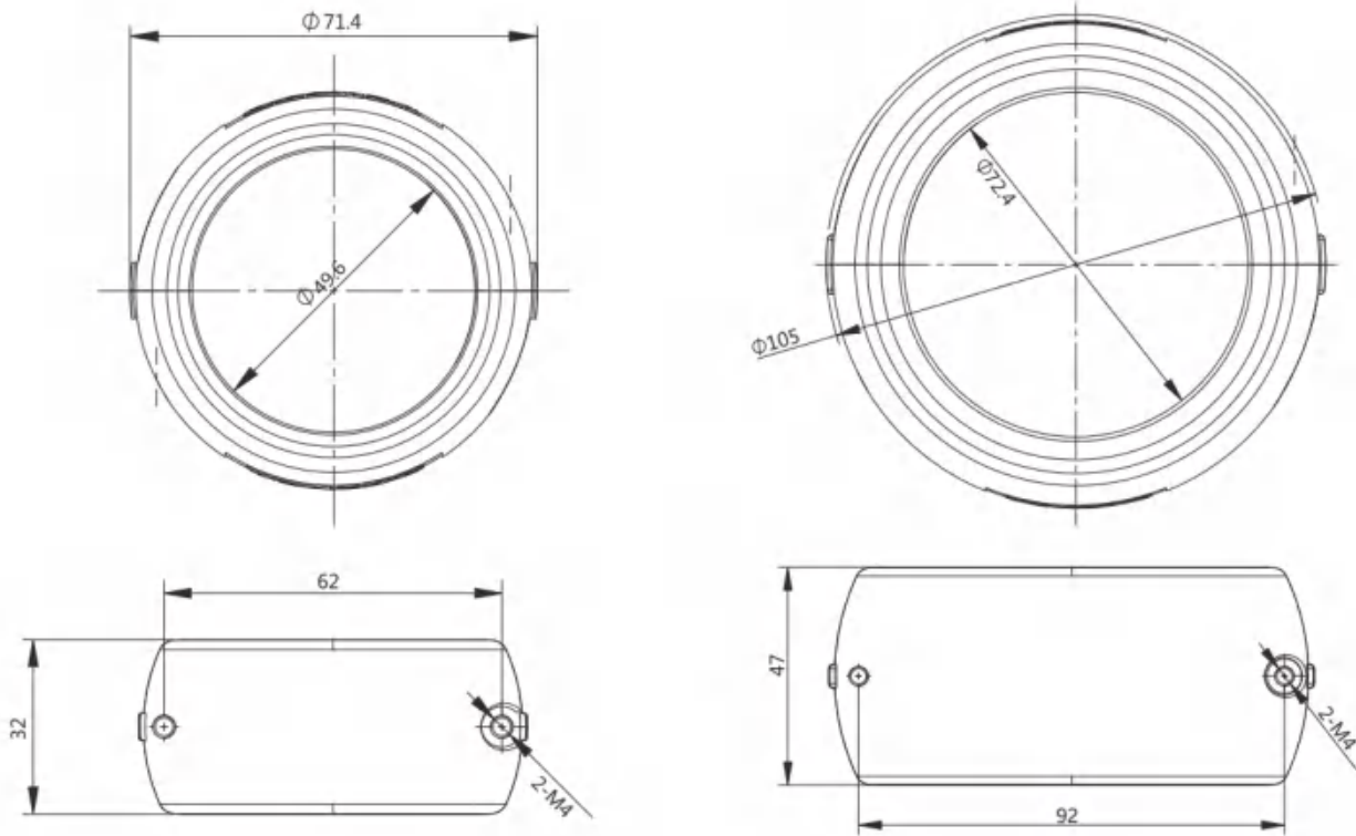
(RGQ-36/48A外形图)
