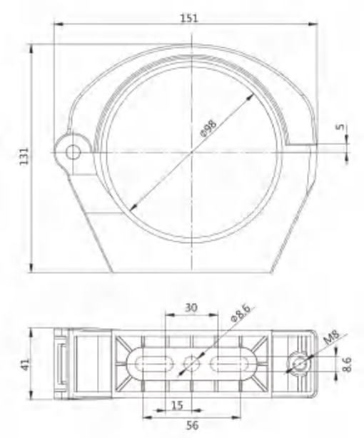
(RGQM-56/70A外形尺寸图)
