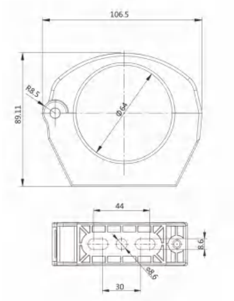
(RGQM-36/48A外形尺寸图)
